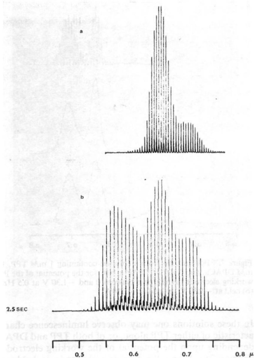
Figure 6. (a) Ecl of TPP-10-MP mixture. The solution contained 1 mM 10-MP, 0.1 mM TPP, and 0.2 M TBAP in MC. Pt electrode cycled at 0.2 Hz between +0.84 ( 10\text{-MP}\cdot^+ production) and -1.26 V ( \text{TPP}\cdot^- production). (b) Ecl of TPP-rubrene mixture. The solution contained 1 mM rubrene, 0.1 mM TPP, and 0.2 M TBAP in MC. Pt electrode cycled at 0.2 Hz between +0.90 \text{R}\cdot^+ production) and -1.26 V ( \text{TPP}\cdot^- production).
