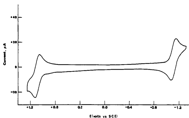
Figure 3. Cyclic voltammogram of TPP at a platinum electrode. The solution contained 1 mM TPP and 0.2 M TBAP in MC. The scan rate was 100 mV/sec.
