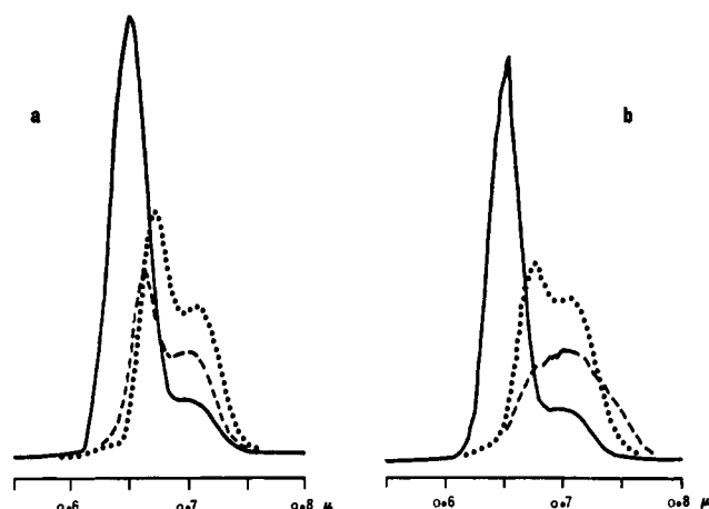
Figure 2. Laser excited fluorescence of TPP: (a) vertical excitation at the geometric center of the cuvette ( \cdots ) 1.00 mM, ( --- ) 0.100 mM, and ( — ) 0.0100 mM TPP solutions in \text{CH}_2\text{Cl}_2 ; (b) vertical excitation positioned for maximum (ca. 7 mm) ( \cdots and --- ) and minimum (ca. 1 mm) ( — ) emission path length in the cuvette; the concentrations and SPF multiplier settings were ( — ) 1.00 mM, 3\times ; ( \cdots ) 1.00 mM, 30\times ; ( --- ) 2.00 mM, 100\times .
