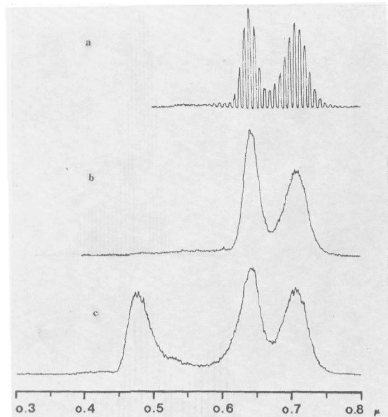
Figure 7. Ecl emission from a solution containing 1 mM TPP, 1 mM DPACl 2 , and 0.100 M TBAP in MC for the potential of the Pt working electrode (a) alternate between 0 and -1.30 V at 0.5 Hz, (b) held at -1.30 V, (c) held at -2.10 V.
